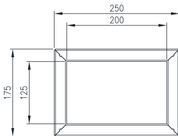
FRONT VIEW MAIN FRAME
