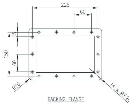
BACKING FLANGE
