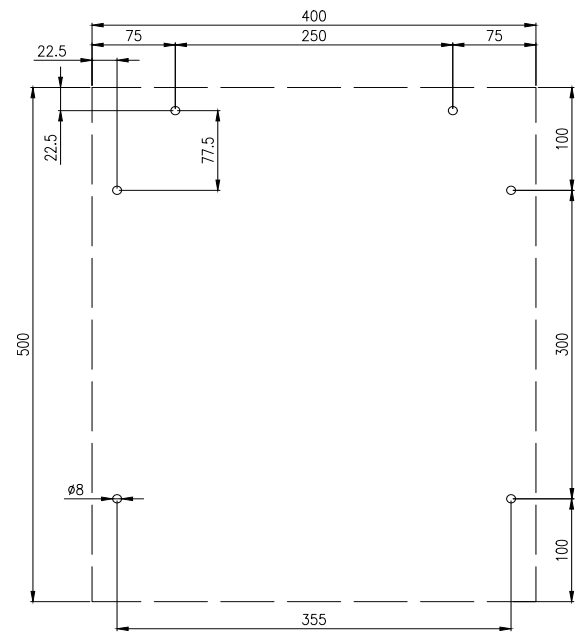
IP-SSVH5040
