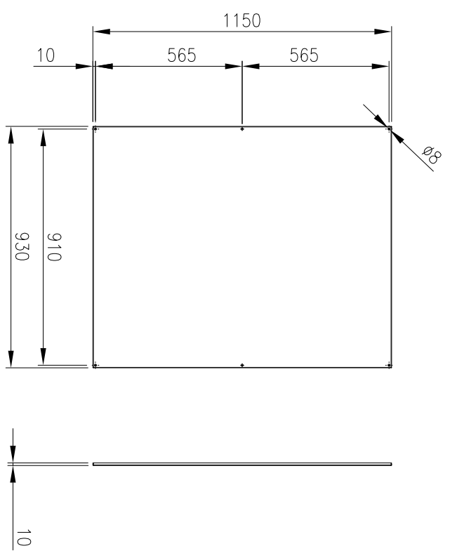
DEVICE MOUNTING PLATE
