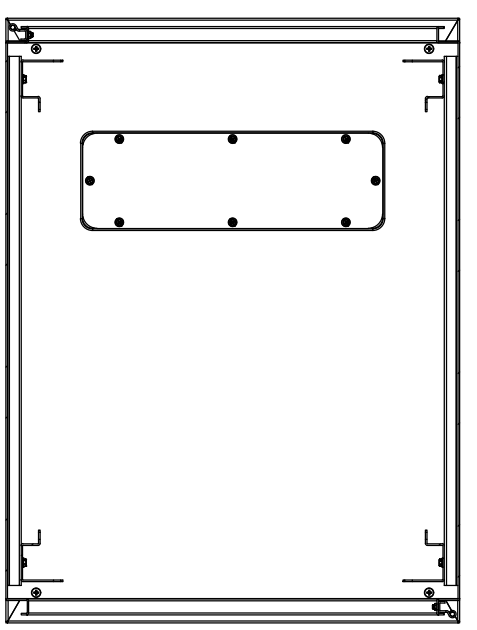
SECTION C-C
