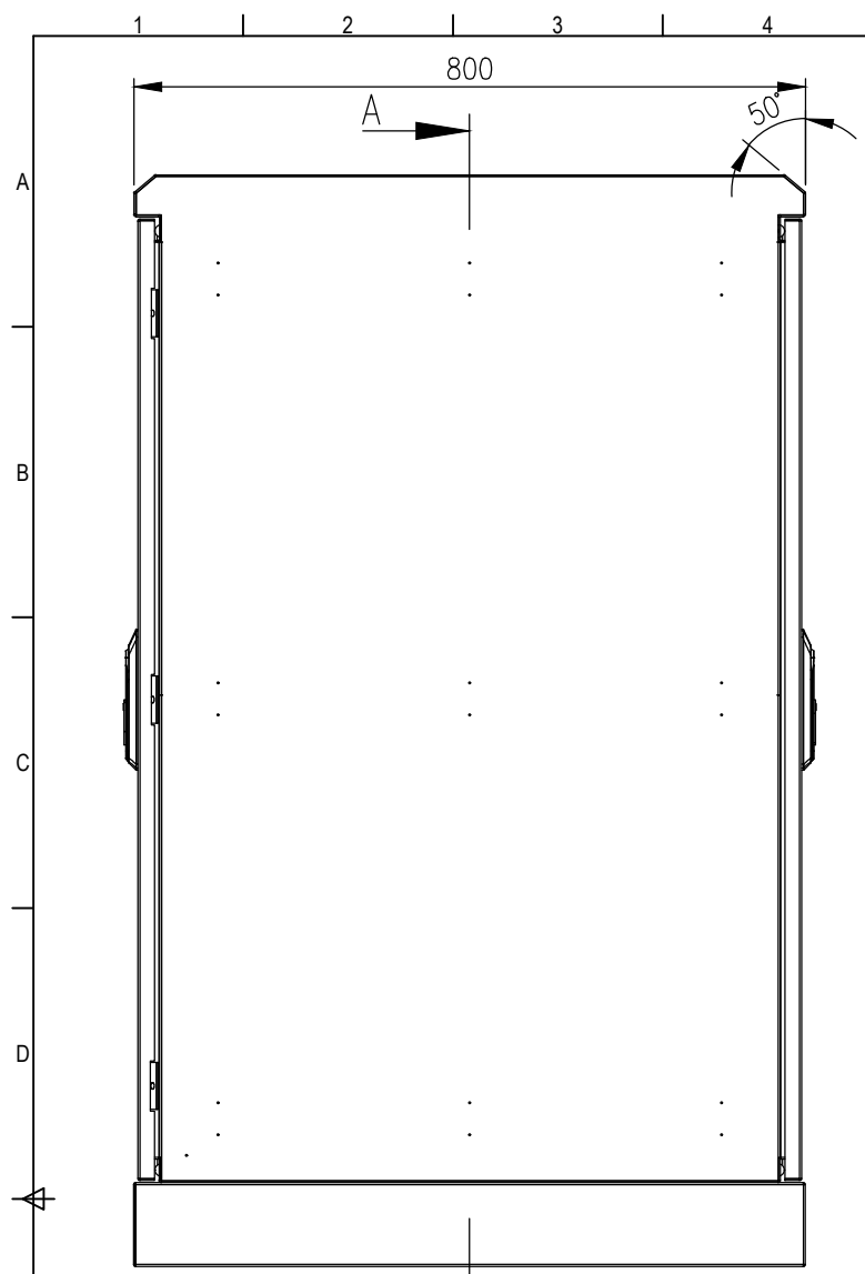
SIDE VIEW
