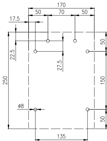
IP-PSVH2517-H
