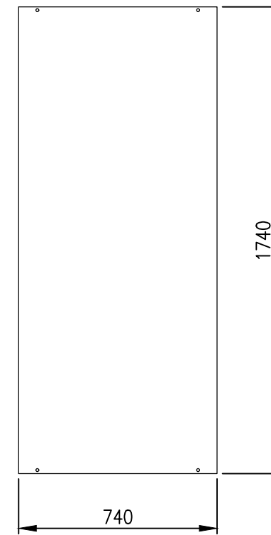
DEVICE MOUNTING PLATE
