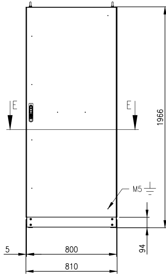
FRONT VIEW (ASSEMBLY)
