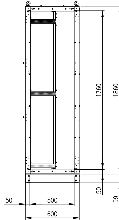
SIDE VIEW (PANELS REMOVED)
