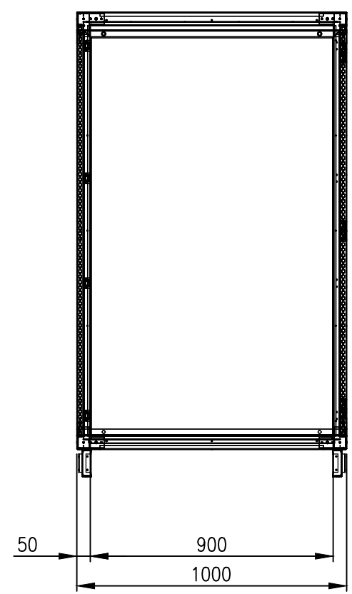
FRONT VIEW (PANELS REMOVED)
