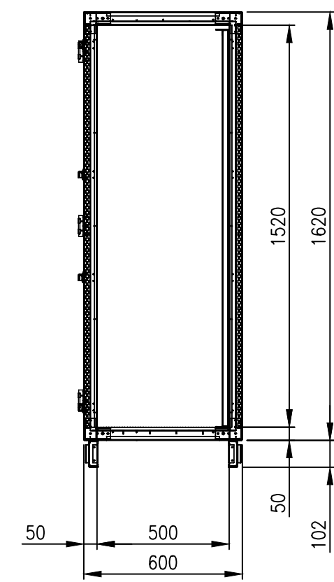
SIDE VIEW (PANELS REMOVED)
