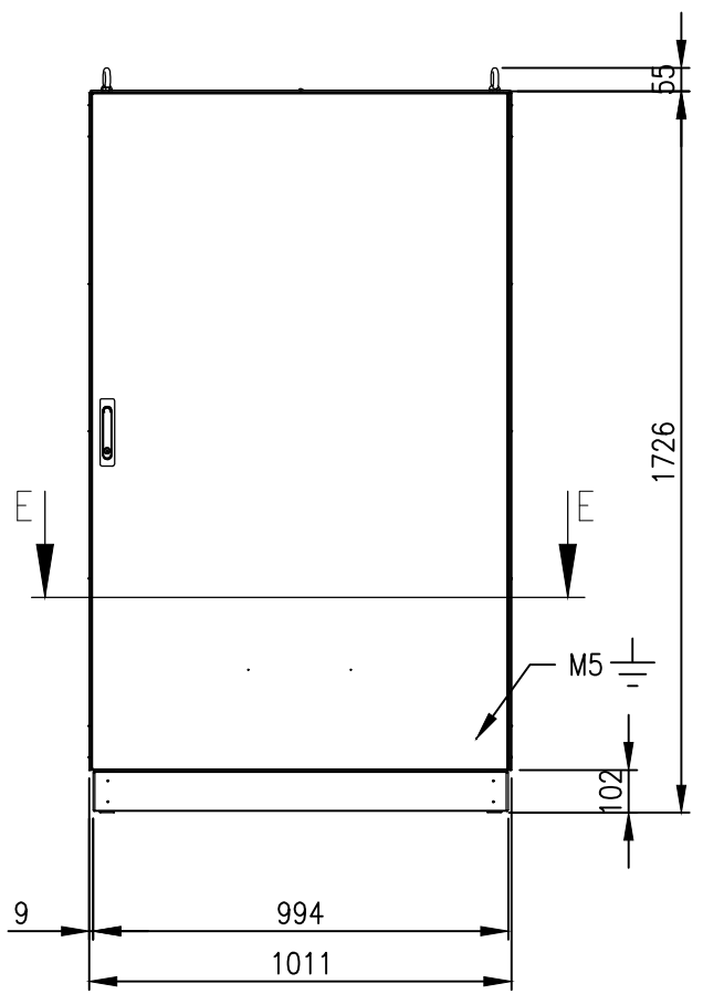
FRONT VIEW (ASSEMBLY)
