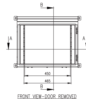
FRONT VIEW-DOOR REMOVED
