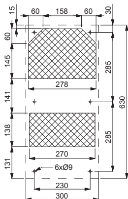
MOUNTING CUT-OUT
