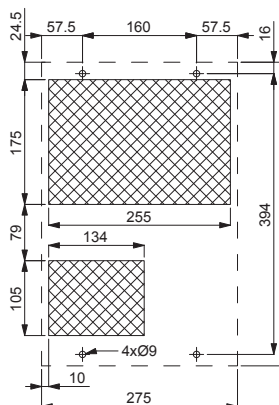
MOUNTING CUT-OUT VIEW FROM EXTERNAL OF ELECTRICAL ENCLOSURE
