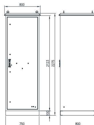
FRONT VIEW (ASSEMBLY)
