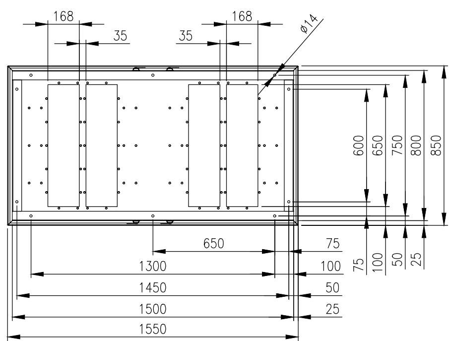
BOTTOM VIEW
