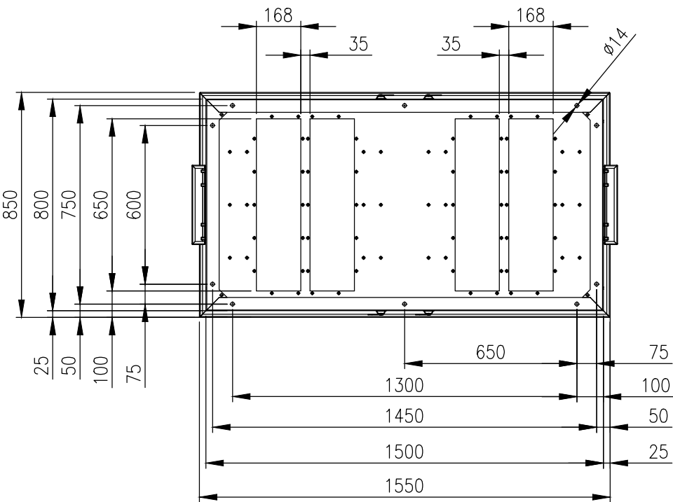
BOTTOM VIEW
