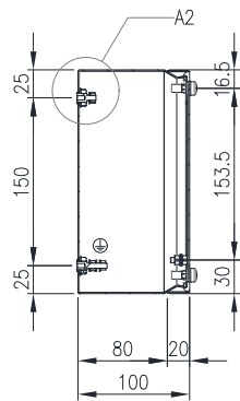
SECTION B-B
