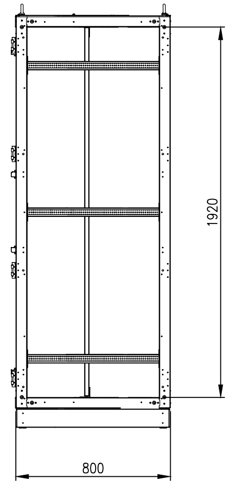
SIDE VIEW (PANELS REMOVED)
