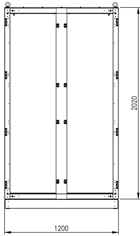
FRONT VIEW (PANELS REMOVED)
