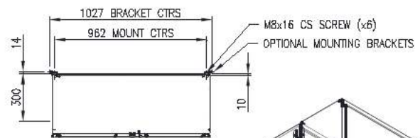
SECTION AW-AW
