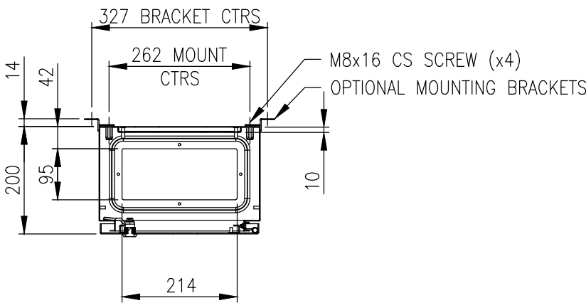
SECTION AW-AW
