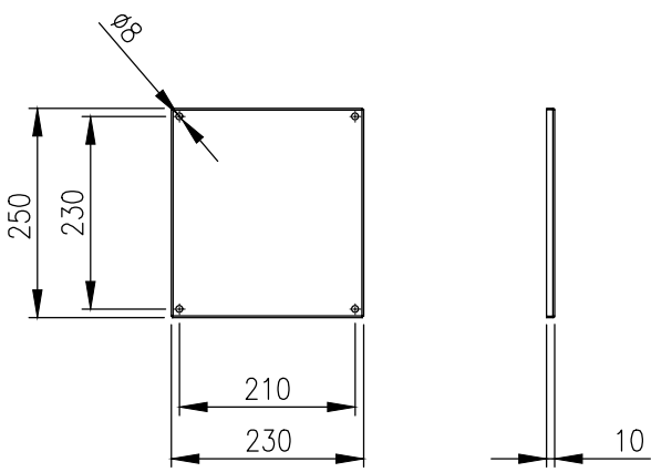
DEVICE MOUNTING PLATE
