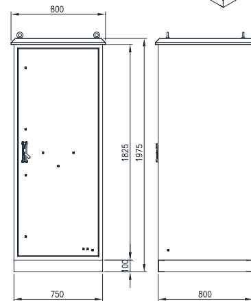
FRONT VIEW (ASSEMBLY)
