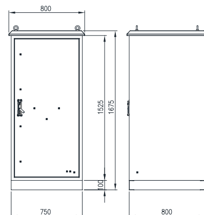
FRONT VIEW (ASSEMBLY)
