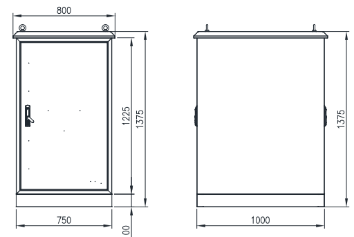
FRONT VIEW (ASSEMBLY)
