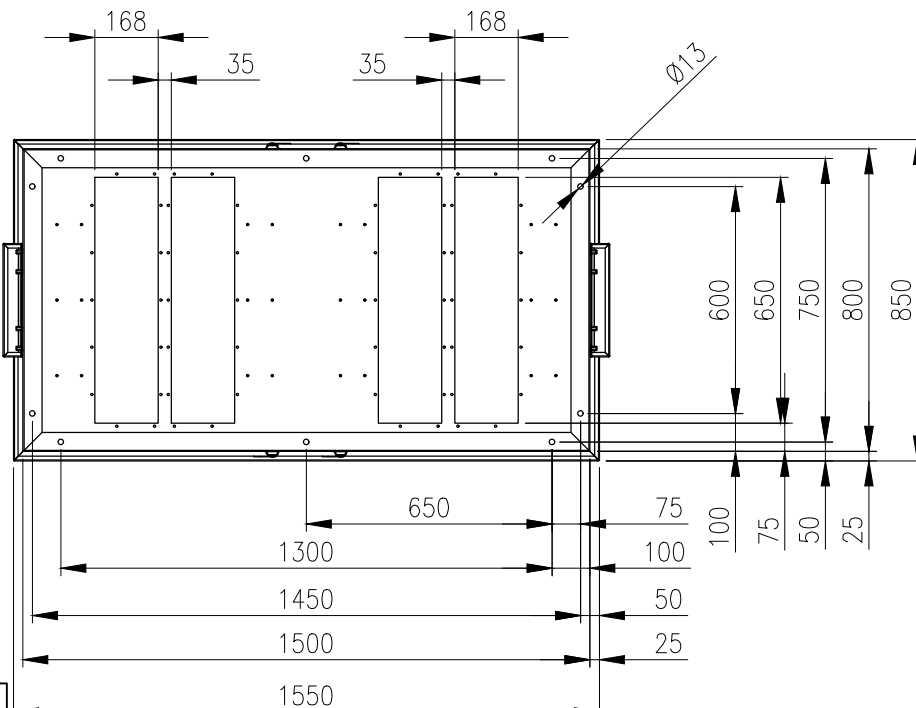
BOTTOM VIEW
