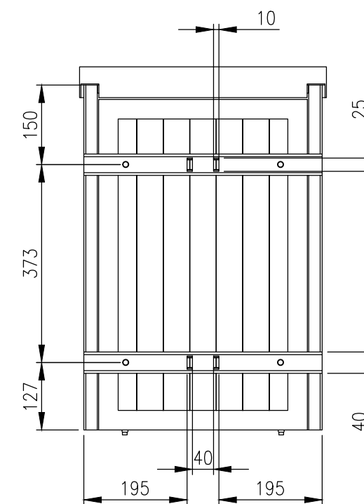
REAR VIEW
