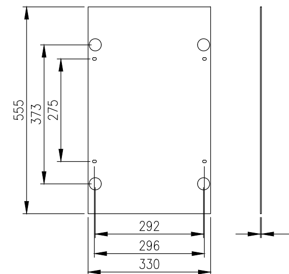
MOUNTING PLATE
