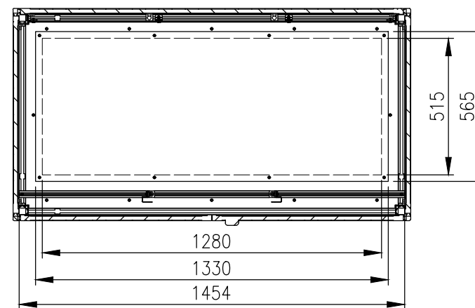
FRONT VIEW—DOOR REMOVED
