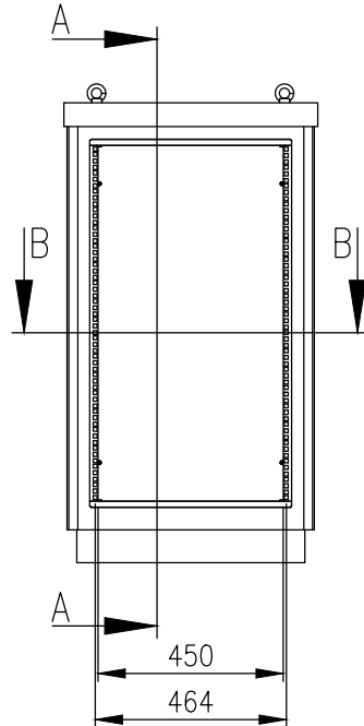
FRONT VIEW-DOOR REMOVED
