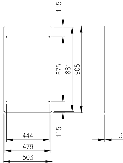
DEVICE MOUNTING PLATE
