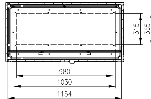
FRONT VIEW—DOOR REMOVED
